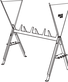
ANT310 260 × 129 × 147/238 cm
