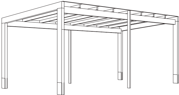
SOP130 320 × 650 × 285 cm
